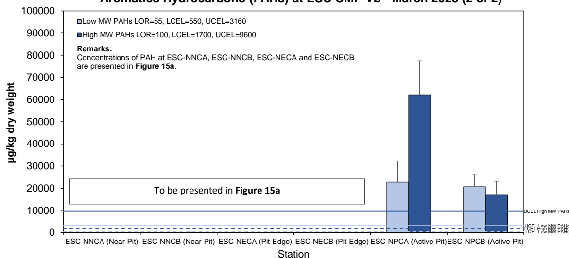
Figure 15b Concentration of Low and High Molecular Weight Polycyclic Aromatic Hydrocarbons ( \mu\text{g/kg} dry weight; mean + SD) in sediment samples collected from Pit Specific Sediment Chemistry Monitoring for ESC CMP Vb in March 2023
