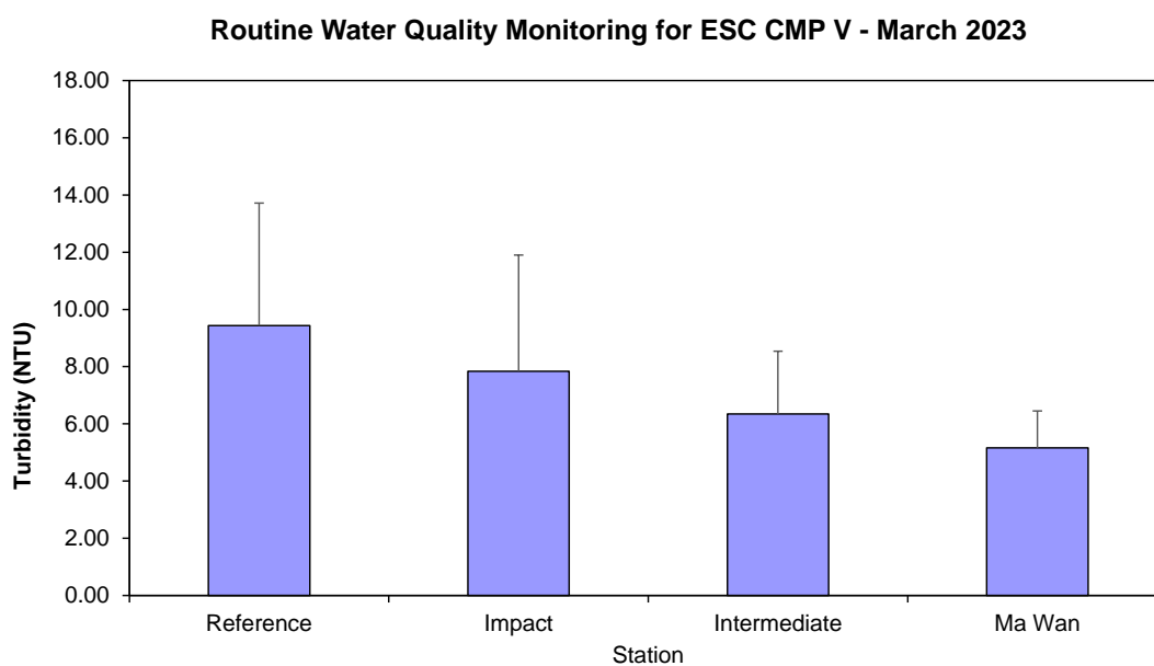
Figure 6: Level of Turbidity (NTU; mean + SD 1 ) recorded during Routine Water Quality Monitoring for disposal operations at ESC CMP V in March 2023
