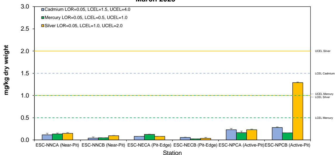
Figure 13: Concentration of Metals (Cd, Hg, Ag; mg/kg dry weight; mean + SD) in sediment samples collected from Pit Specific Sediment Chemistry Monitoring for ESC CMP Vb in March 2023
