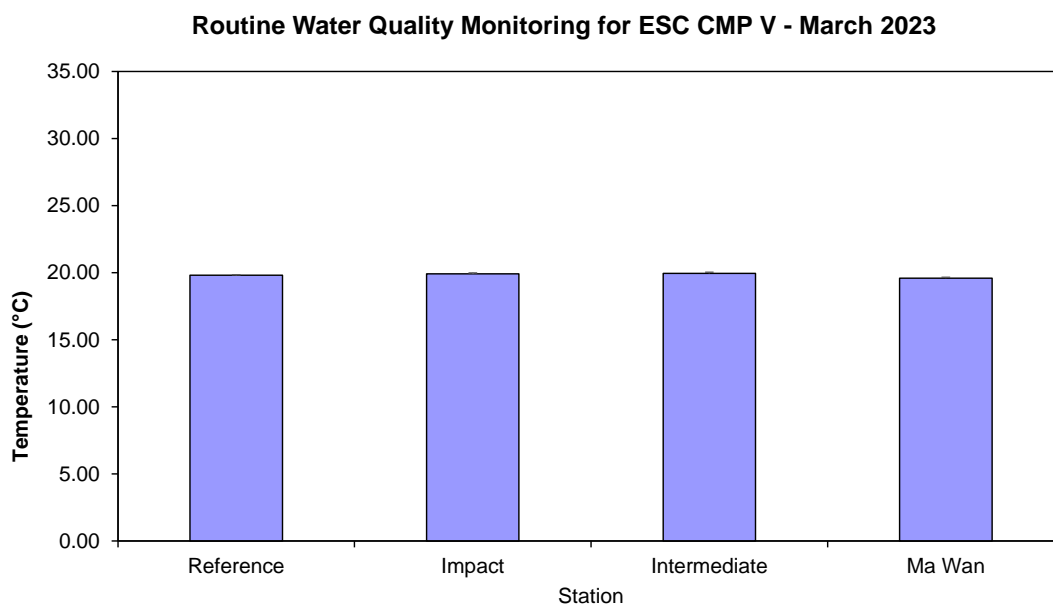
Figure 4: Level of Temperature (°C; mean + SD 1 ) recorded during Routine Water Quality Monitoring for disposal operations at ESC CMP V in March 2023
