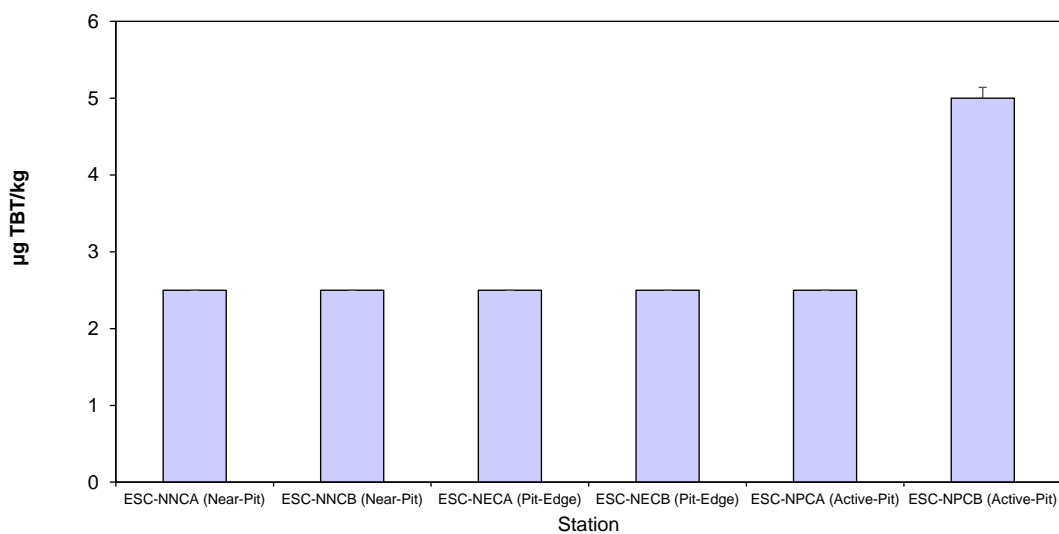
Figure 16: Concentration of Tributyltin (TBT) (µg TBT/kg; mean + SD) in sediment samples collected from Pit Specific Sediment Chemistry Monitoring for ESC CMP Vb in March 2023
