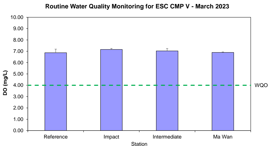
Figure 3: Concentration of Dissolved Oxygen (DO) (mg/L; mean + SD 1 ) recorded during Routine Water Quality Monitoring for disposal operations at ESC CMP V in March 2023
